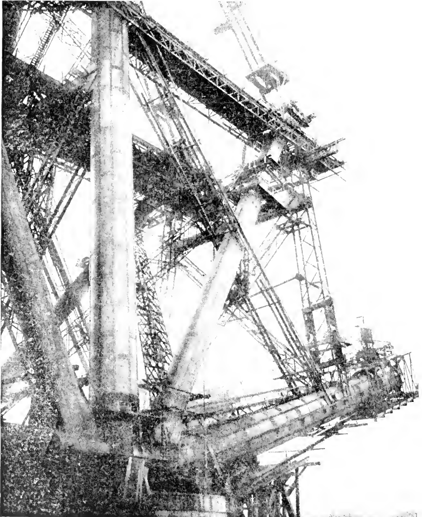
CONSTRUCTIONAL DETAIL OF THE FORTH BRIDGE
